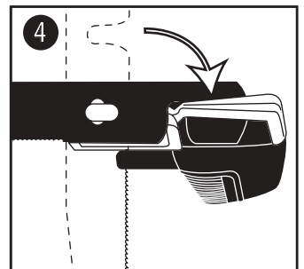
LEFT CUTTING POSITION
